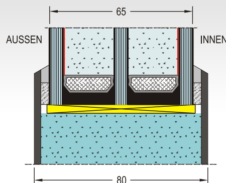
ISOGLAS U_g = 0,5 \text{ W/m}^2\text{K}
