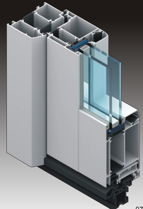
ISOGLAS - U_g = 1,1 \text{ W/m}^2\text{K}
